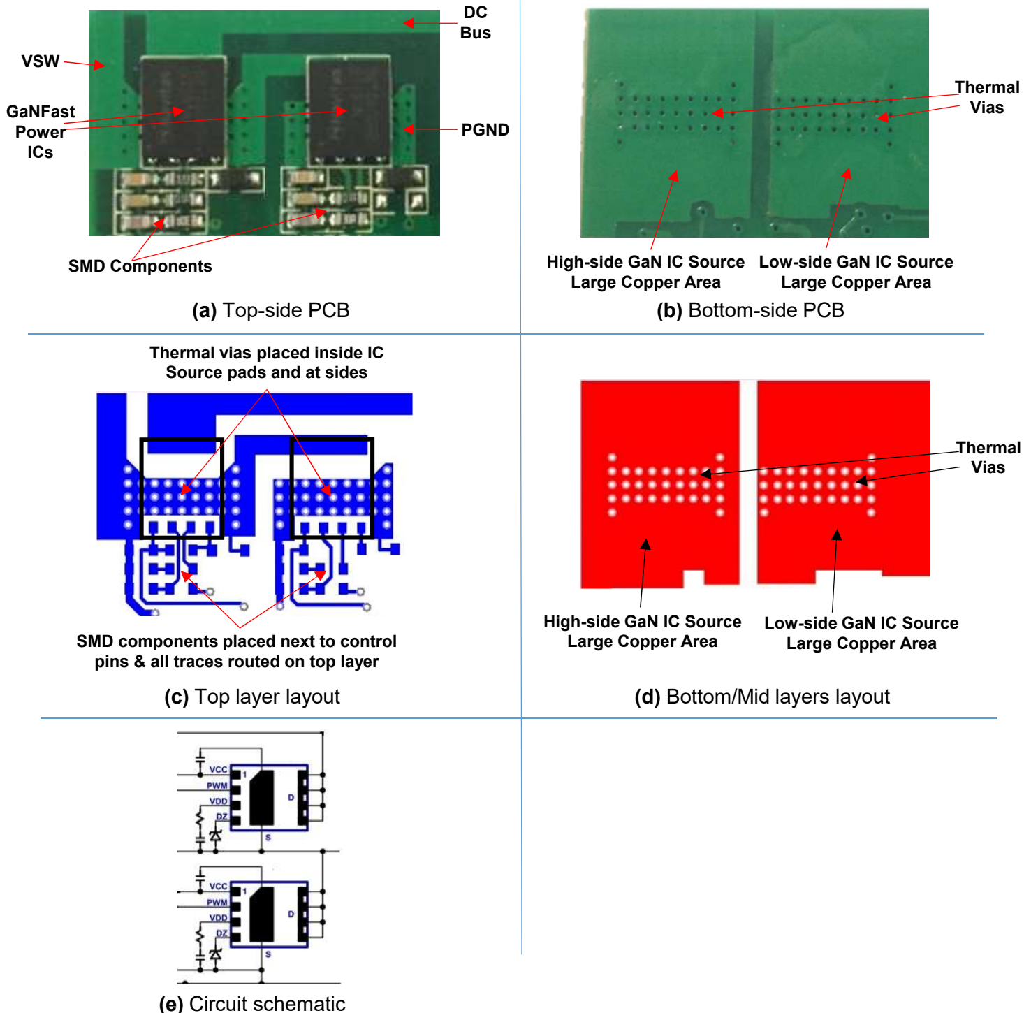
Fig 4. PCB and layout for GaN Power ICs in half-bridge configuration.
