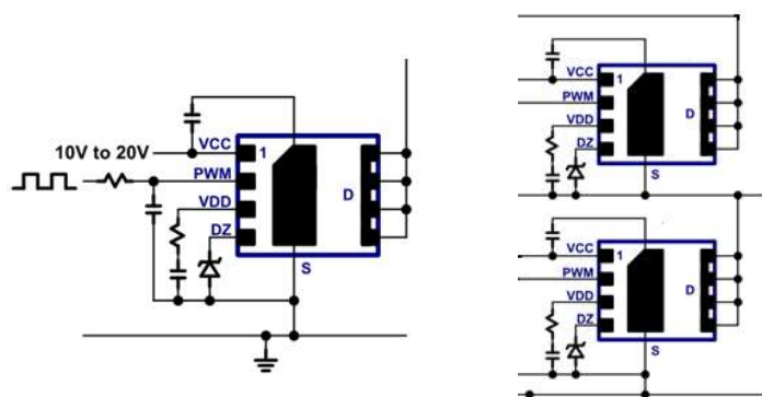
(e) Circuit schematic
