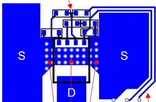
Thermal vias placed inside IC Source pad and at sides Route signal lines around Cu areas
