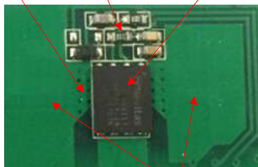
Source PGND Drain Large Cu areas VCC & PWM
