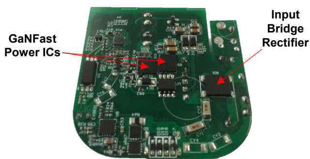
(a) 45 W charger bottom side PCB
