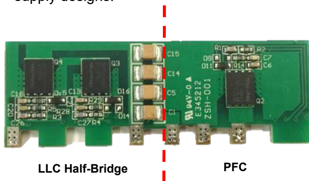
(a) Top-side PCB
