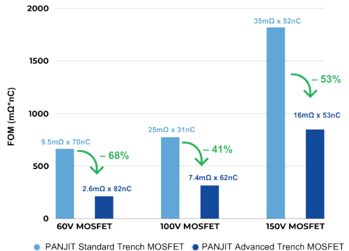
FOM - Standard vs. Advanced Trench
